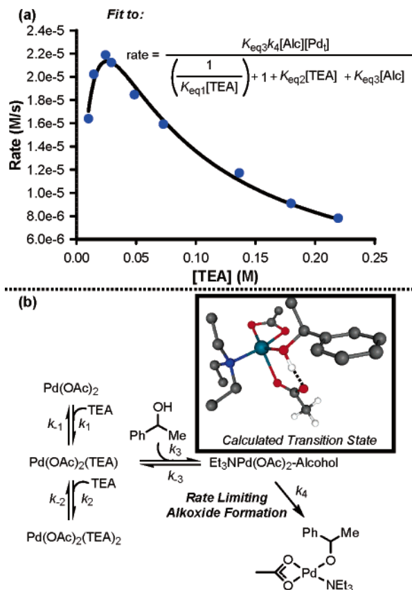
FIGURE 3. (a) Rate dependence on [TEA]. (b) Rate-limiting alkoxide formation with a single TEA ligand.
